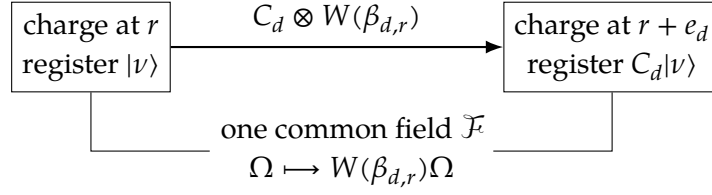
Figure 1: The charged step acts on the register and field together. Each of the six incident field prices acts on this same field space.
