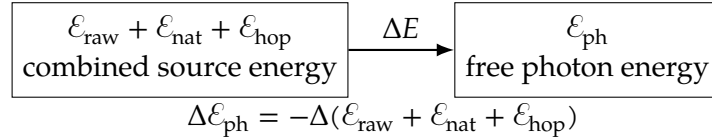
Figure 2: The exact exchange concerns the combined source terms. Its identity allows individual terms to increase while their sum decreases.
