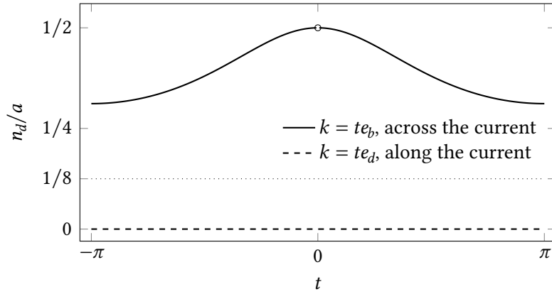
Figure 7.3. The coupling density n_d of unit currents of direction d , in units of a , along the current's own axis (dashed, zero for t \neq 0 ) and along another axis (solid, \omega(2 - 2 \cos t) , between \text{arsinh}(1)/(2\sqrt{2}) \approx 0.3116 at t = \pm\pi and 1/2 as t \rightarrow 0 ). The two limits at k = 0 differ, so no trigonometric polynomial agrees with the density near k = 0 , and infinitely many of its Fourier coefficients, the static couplings, are nonzero. The dotted line marks the bound a/8 used in the proof.
