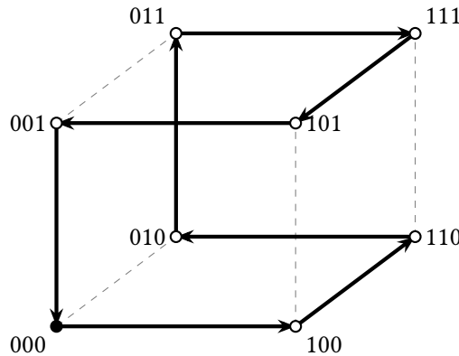
Figure 4.1. The parity patterns of three accounts are the corners of a cube; each post moves the pattern along one edge, the first bit for account 1. Thick arrows: the reflected binary tour (4.4), which occupies every corner and closes in eight ticks. Dashed: the four edges it does not walk, one at each corner. The empty pattern 000 is filled. Twelve tours leave 000 (Theorem 4.9).
