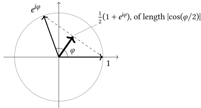
Figure 7.1. What one other register does to a coherence. When register p changes its occupation, the occupied half of q acquires the interaction phase e^{i\varphi} and the empty half does not, so the coherence of p is multiplied by the average of the two unit vectors (thick arrow), of length |\cos(\varphi/2)| .
