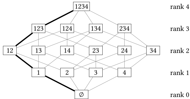
Figure 5.1. The record cell. Each box is a record, labelled by the set of accounts that hold a posting; lines join records that differ by one posting. The thick chain is the history that posts accounts 1, 2, 3, 4 in that order. The 24 histories are the 24 chains from the empty record at the bottom to the full record at the top, and each is a simplex of the chain subdivision of the four-cube (Theorem 5.2).
