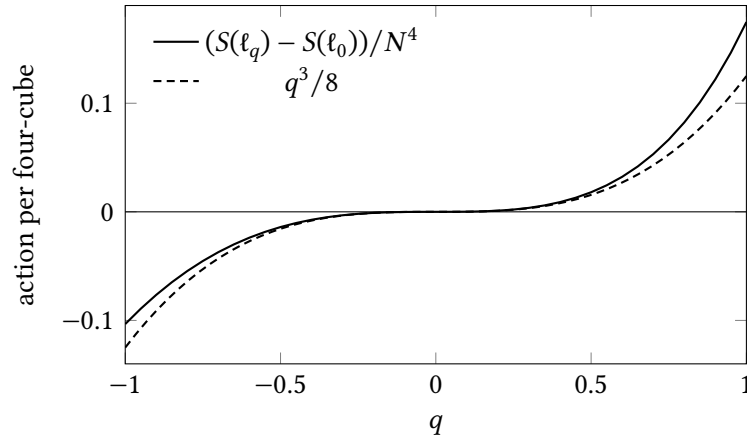
Figure 5.2. The change of Regge's action per four-cube along the body path, computed by numerical integration of the closed form of F in Theorem 5.16 (solid), and its cubic germ q^3/8 (dashed). The curve crosses its flat value with zero slope and zero curvature: flatness is stationary and is neither a minimum nor a maximum (Corollary 5.17).
