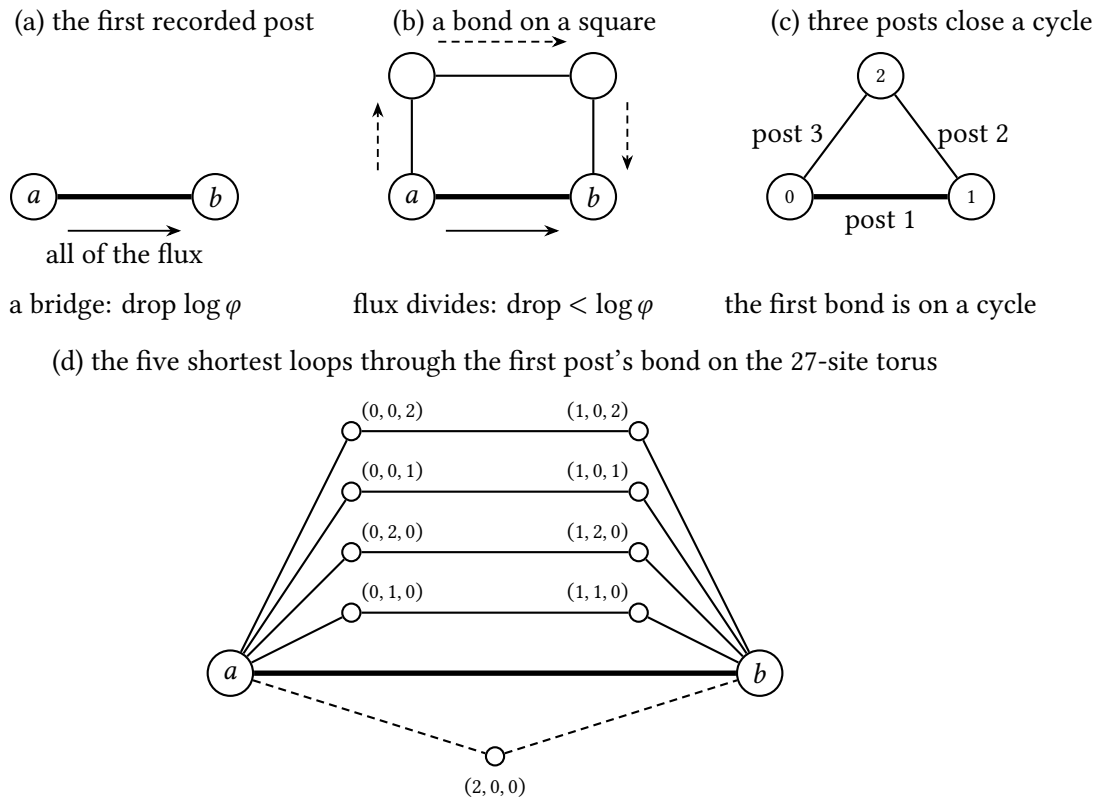
Figure 3.1. Carriers of a post's field; the thick bond is the post's own bond, from a to b . (a) The record carrier of the first post is one bond, a bridge, so the whole flux crosses it. (b) On a square part of the flux goes round (dashed arrows) and the drop falls. (c) On the 27-site torus three forward posts along one axis close a cycle through the first bond (Proposition 3.31). (d) On the possibility graph on T_3 , with a = (0, 0, 0) and b = (1, 0, 0) , the triangle through (2, 0, 0) (dashed, it wraps round the period) and four squares; they share no bond, and together they use every bond at a and at b (Corollary 3.53).
