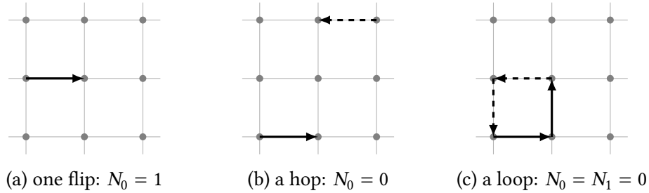
Figure 7.5. Flip patterns in one plane, with e_0 to the right and e_1 upward. A solid arrow marks a block that fills the register on its edge (current +1 along the edge), a dashed arrow a block that empties it (current -1, drawn in the direction the current flows). N_d = \sum_{p=d} \delta_p is the net current along e_d . (a) One flip carries a net current. (b) A hop carries none. (c) The four flips around a plaquette carry no net current along either direction and circulate without divergence. All three have a nonzero transverse part and lose their value on time average on an assignment that fills the directions they use (Theorem 7.47). The star of Figure 7.4 has no net current either, but it is a gradient and is conserved.
