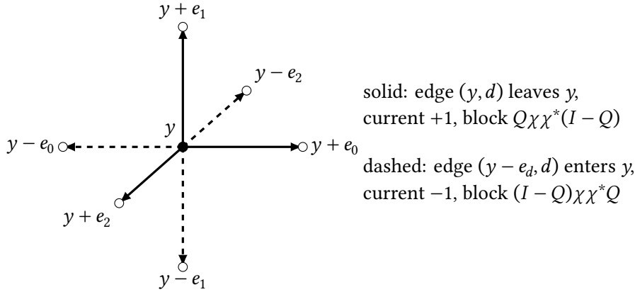
Figure 7.4. The star of a site y . The gradient \nabla 1_y is +1 on the three edges leaving y (solid) and -1 on the three entering it (dashed), so it flows outward along all six (arrows) and has no transverse part. Registers on these edges, flipped in the pattern of this current, form a joint coherence that the field cannot see: its reference value stays 4^{-6} at all times, although each flip alone averages to zero.
