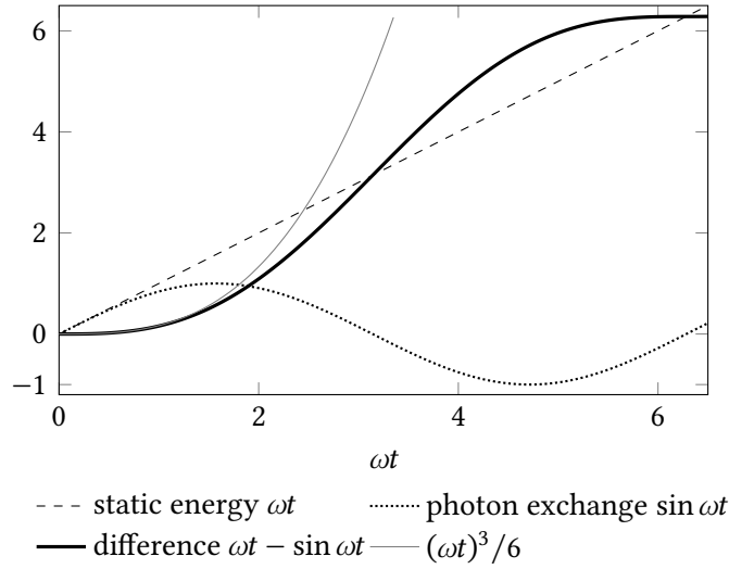
Figure 7.2. The time factor of the phase kernel at one photon frequency \omega : static energy \omega t (dashed) less photon exchange \sin \omega t (dotted). The difference (thick) starts as (\omega t)^3/6 (thin gray) and stays between zero and that cubic for t \geq 0 .
