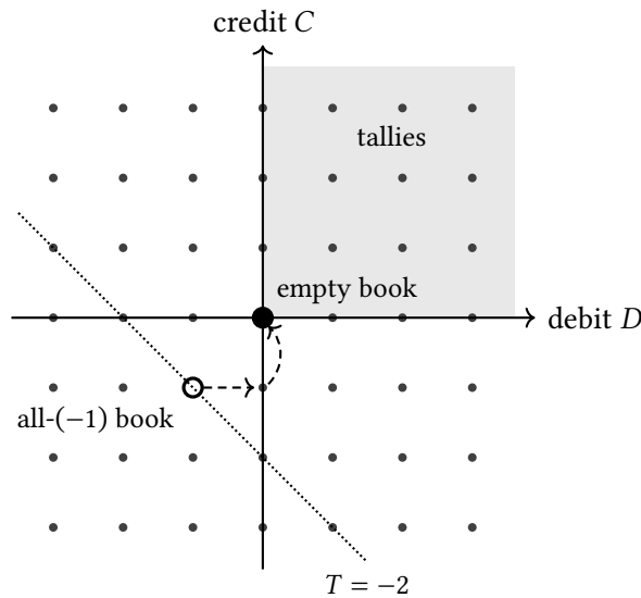
Figure 2.2. Books for one account as integer points (D, C) . Posting steps move one unit right (debit) or up (credit), with the same shape everywhere. The shaded quadrant of nonnegative counts is the set of tallies. The shift by -1 carries the empty book (filled) to the all- (-1) book (open), which is the tally of no record, has total T = -2 , and reaches the empty book in two posts (dashed).
