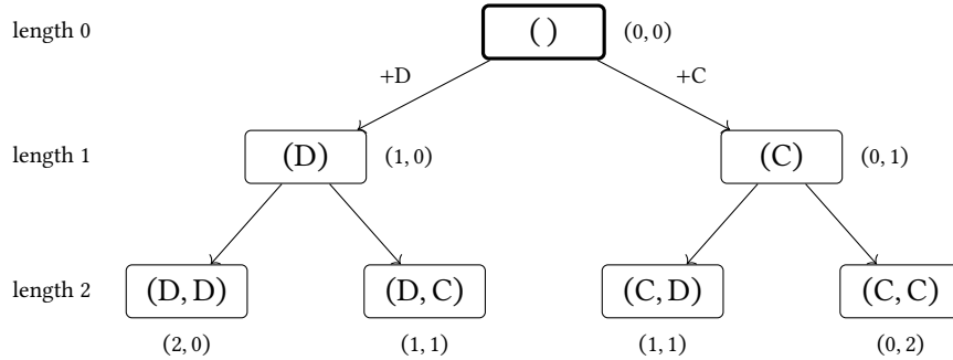
Figure 2.1. Records over one account ( d = 1 ) up to length two, each with its tally (D, C) . The empty record (thick box) is the root; every record has a successor one post longer, and nothing precedes the root. The records (D, C) and (C, D) differ and write the same book.
